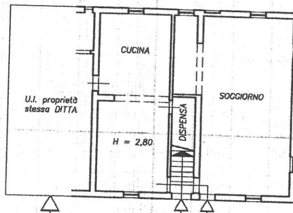
PIANO TERRA
